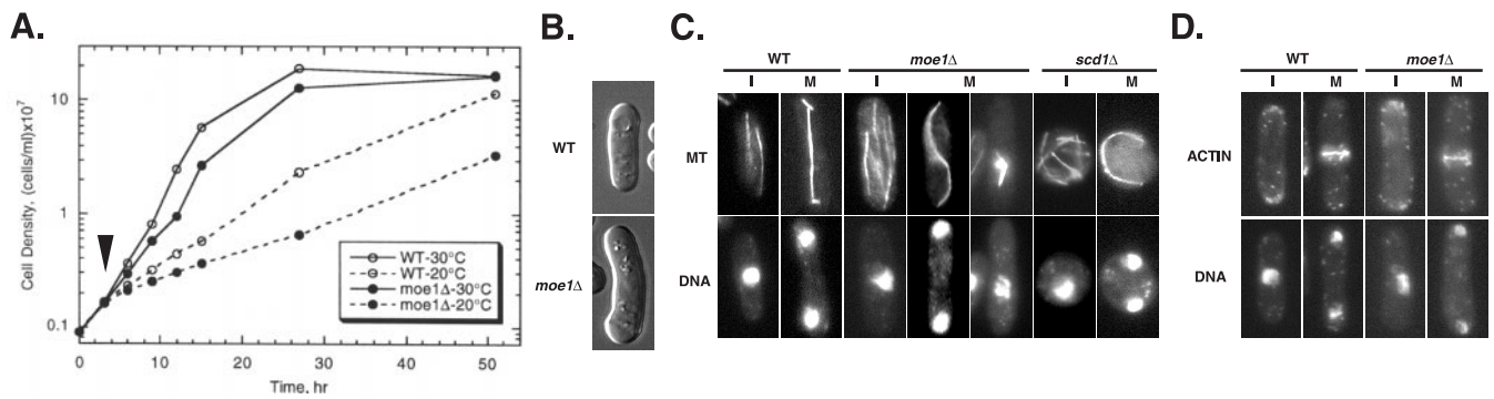
FIG. 1. Growth curve, cell morphology, and MTs of various strains. (A) Cells were grown to \approx 4 \times 10^6 cells/ml at 30°C and then diluted to 1 \times 10^6 cells/ml at t = 0 . After 3 hr (marked by an arrow), cells either were transferred to 20°C or remained at 30°C, and the cell density was monitored over time. (B) Cells were pregrown in solid rich medium at 30°C for 24 hr before being examined. The frequency of bent cells was 20%. (C and D) Cells were grown at 20°C to mid-log phase and subjected to fluorescence microscopy to visualize MTs, F-actin, and DNA. scd1Δ and ras1Δ cells showed the same abnormal phenotype in MTs at 30°C. I, interphase; M, mitosis. Strains used: SP870 (wild type, WT), MOE1U ( moe1Δ ), SPSCD1U ( scd1Δ ), and SPRN ( ras1Δ ).
